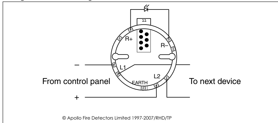
Fig 4 UV Flame Detector base connections
